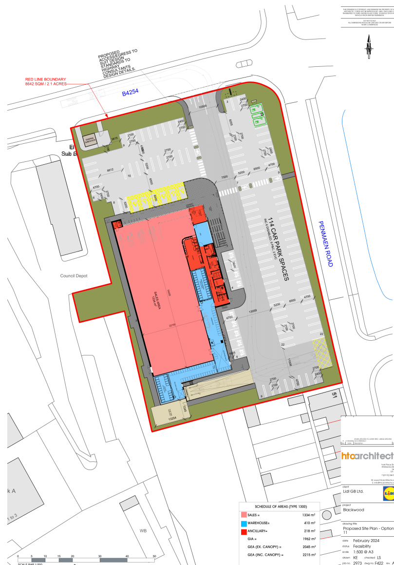
FIGURE 2: PROPOSED DEVELOPMENT LAYOUT
